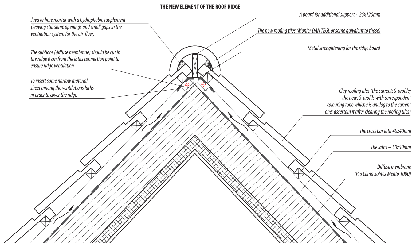
Roof with a ventilation system. The current constructions and the applicable additional materials, their characteristics, to develop an insulated roof with a ventilation system. A drawing among the project materials 20
